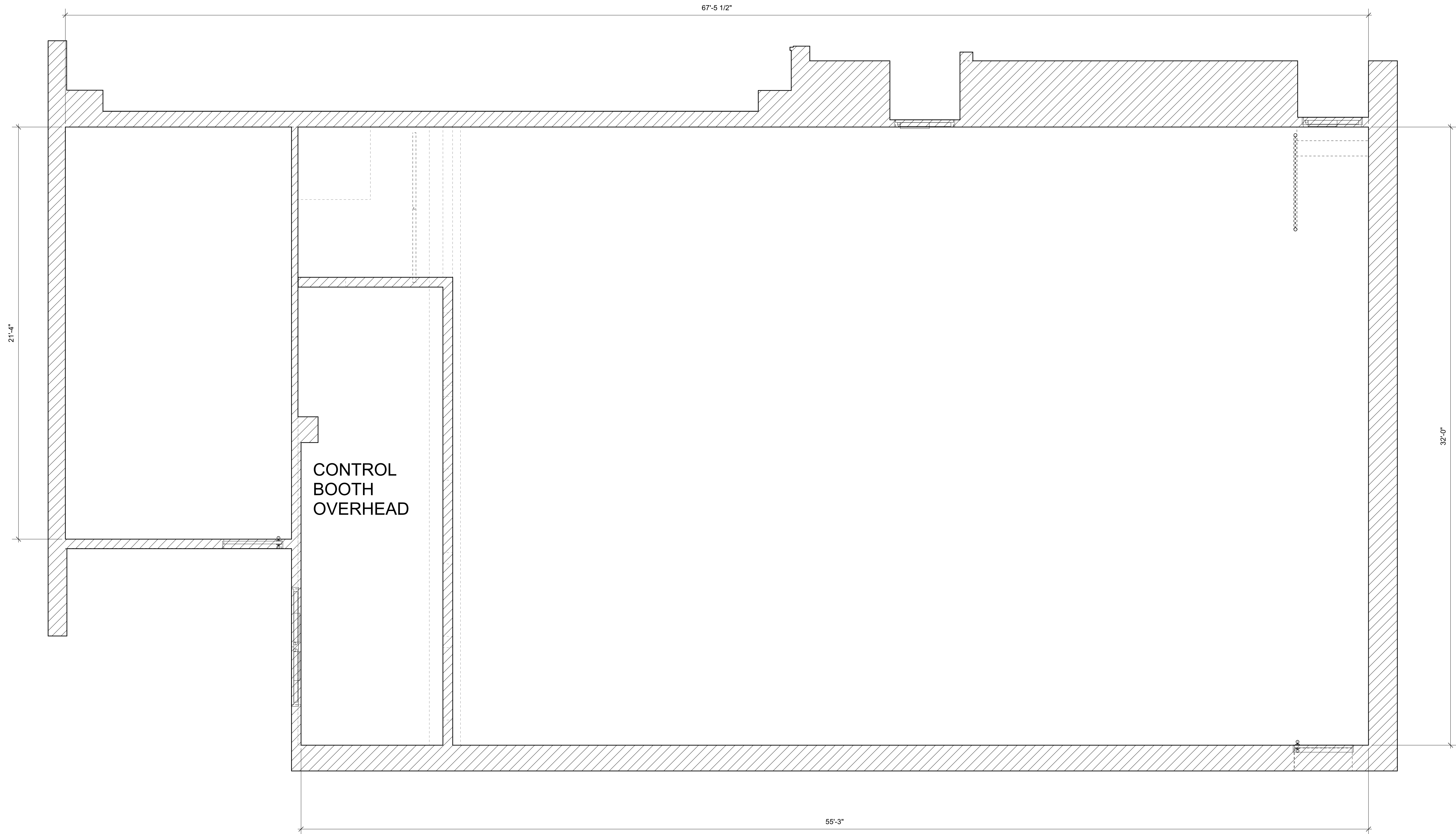
1 GROUND PLAN Scale: 3/8" = 1'-0"
