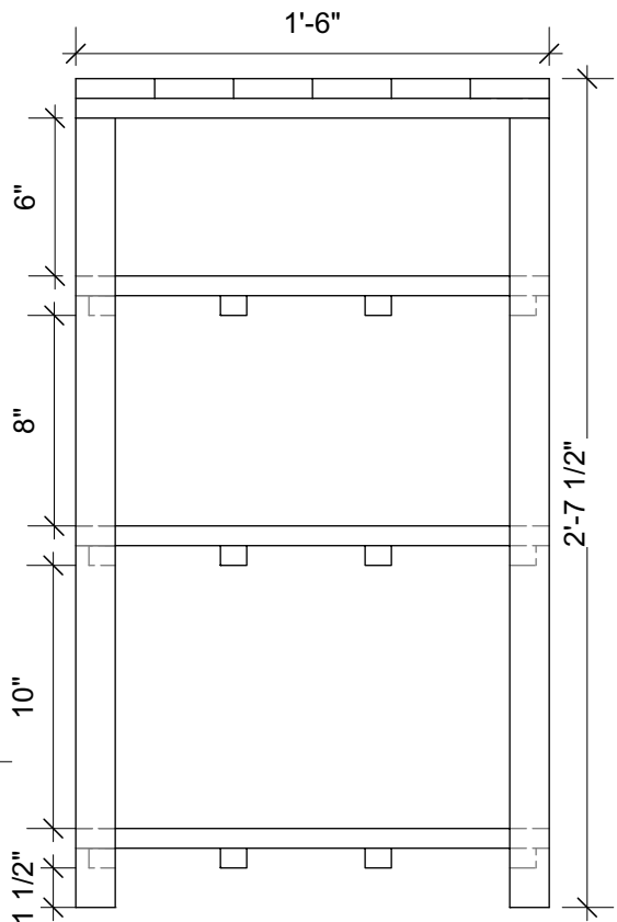
3 Desk Right View Scale: 1 1/2" = 1'-0"
